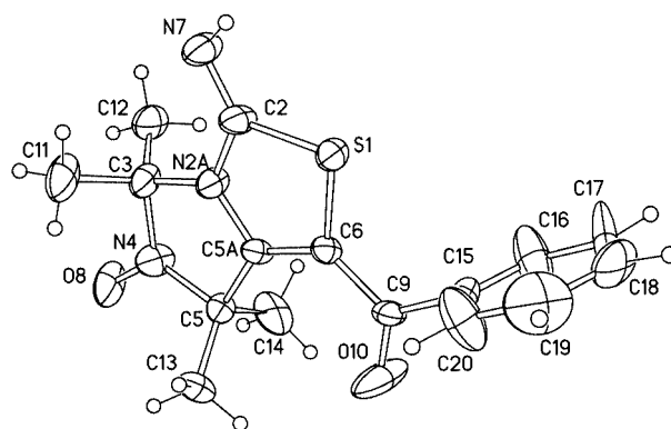
Figure 1. Crystal structure of radical 7a ; selected bond lengths [Å]: S1–C2 1.765(4), S1–C6 1.761(4), C2–N2a 1.398(5), N2a–C3 1.477(5), N2a–C5a 1.357(5), C3–N4 1.484(6), N4–C5 1.478(6), N4–O8 1.263(4), C5–C5a 1.512(5), C5a–C6 1.361(6)
